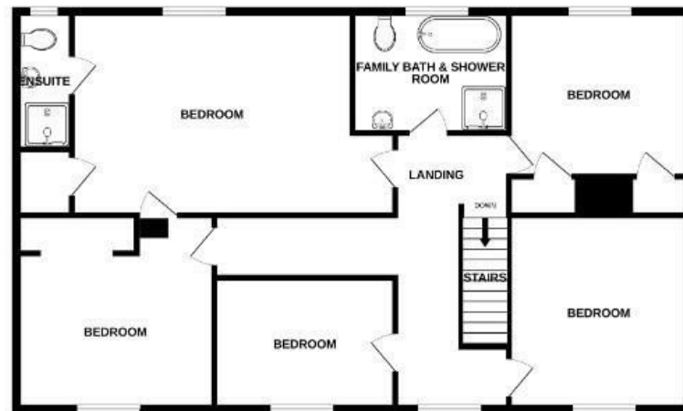
1ST FLOOR 1180 sq.ft. (109.6 sq.m.) approx.
