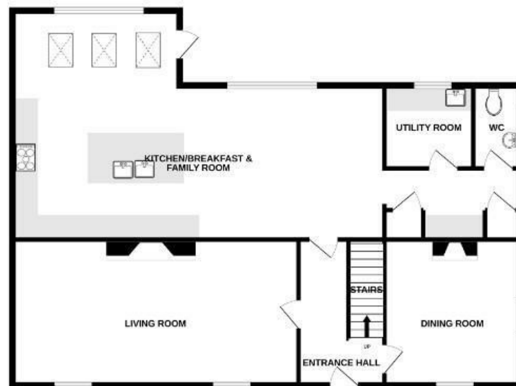
GROUND FLOOR 1270 sq.ft. (118.0 sq.m.) approx.
